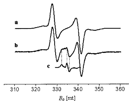
Figure 8. Simulated (a) and experimental (b) EPR spectra of dilabelled hexapeptide 11 . Trace (c) is the spectrum of monolabelled tetrapeptide 10 . The two experimental spectra were obtained in frozen MeOH solution at 120 K (peptide concentration: 1 mm).
