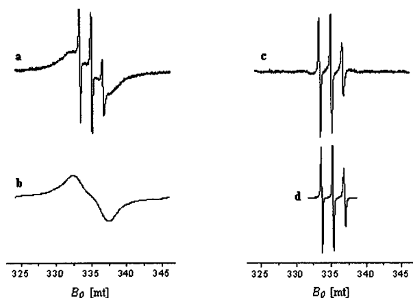
Figure 7. Analysis of the EPR spectrum (a) of dilabelled hexapeptide 11 . The sharp component (c) was obtained by subtracting the broad component (b) from spectrum (a). Trace (d) is the EPR spectrum of monolabelled tetrapeptide 10 . The two experimental spectra were obtained in liquid MeOH solution at 258 K (peptide concentration: 1 mm).
