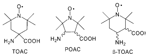
Figure 1. Chemical structures of the spin-labelled amino acids TOAC, POAC and \beta -TOAC.
