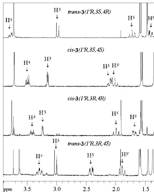
Figure 3. ^1\text{H} NMR spectra ( \text{D}_2\text{O} ) of the diastereomers 3 · \text{HCl} after nitroxide reduction.
