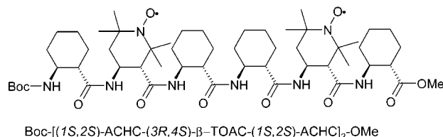
Figure 4. \beta -Hexapeptide 11 containing two (3 R ,4 S )- \beta -TOAC residues at positions 2 and 5 (Boc is tert -butyloxycarbonyl).
