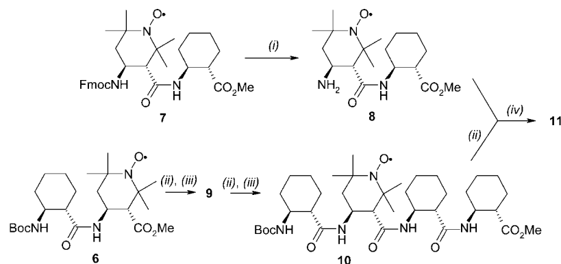
Scheme 5. Synthesis of hexapeptide 11 . (i) \text{CH}_3\text{CN}/\text{Et}_2\text{NH} , 9:1; room temp.; 2 h. (ii) \text{NaOH} (aq), \text{MeOH} , reflux. (iii) \text{H}-(1\text{S},2\text{S})\text{-ACHC-OMe} , EDC, HOAt, DIEA, \text{CH}_2\text{Cl}_2 , 0 °C to room temp. (iv) EDC, HOAt, DIEA, \text{CH}_2\text{Cl}_2 , 0 °C to room temp., 18 h.
