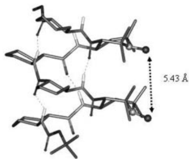
Figure 9. Model of hexapeptide 11 in the 3_{14} -helical structure, which highlights the distance between the oxygen atoms of the nitroxyl probes of the two (3 R , 4 S ) \beta -TOAC residues.
