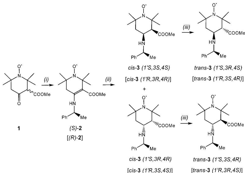
Scheme 1. (i) ( S )- [or ( R )]- \alpha -methylbenzylamine, AcOH, EtOH, 4-Å MS, room temp., 48 h. (ii) NaBH 3 CN, AcOH, EtOH, 75 °C, 2 h; then HCl/EtOAc, 0 °C, filtration and recrystallisation from MeCN. (iii) NaOMe, MeOH, 70 °C, 18 h.
