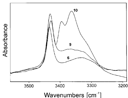
Figure 5. FTIR absorption spectra in the amide N–H stretching region of the Boc/OMe terminally protected, N-terminal, synthetic intermediates of hexapeptide 11 : dipeptide 6 , tripeptide 9 and tetrapeptide 10 in \text{CDCl}_3 solution (peptide concentration: 1 mM).
