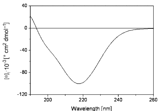
Figure 6. Far-UV CD spectrum of hexapeptide 11 in MeOH solution (peptide concentration: 1 mm).
