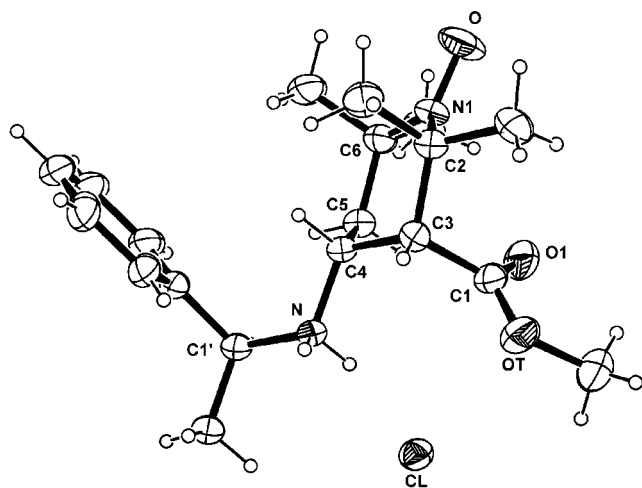
Figure 2. X-ray diffraction structure of cis - 3 ( 1'S,3R,4R ) hydrochloride with selected atom numbering. Displacement ellipsoids for non-hydrogen atoms are drawn at the 30% probability level.
