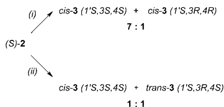
Scheme 2. Reduction of enamine ( S )- 2 . (i) NaBH 4 , AcOH, EtOH, 0 °C to room temp., 7 h. (ii) NaBH 4 , (CH 3 ) 2 CHCOOH, toluene, 0 °C to room temp., 24 h.
