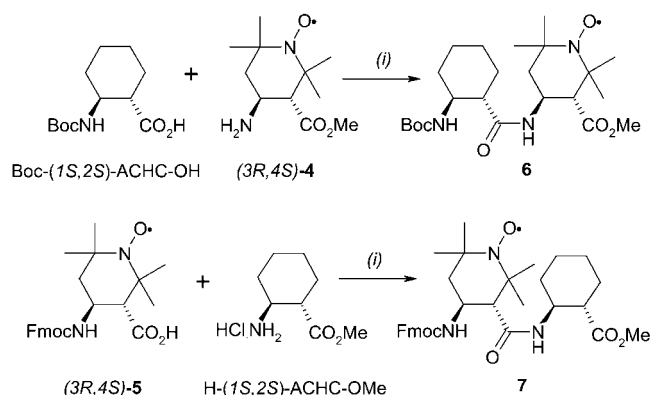
Scheme 4. Synthesis of dipeptides 6 and 7 . (i) EDC, HOAt, DIEA, CH 2 Cl 2 , 0 °C to room temp., 18 h {EDC, N -ethyl- N' -(3'-(dimethylamino)propyl)carbodiimide; HOAt, 7-aza-1-hydroxy-1,2,3-benzotriazole}.
