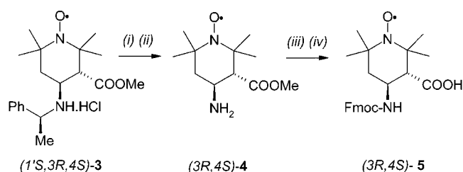
Scheme 3. Removal of the chiral auxiliary from diastereomers 3 , followed by C-deprotection/N-protection of resulting \beta -amino ester enantiomer 4 . (i) H 2 , Pd/C 10%, 95% EtOH, room temp., 30 min. (ii) Cu(OAc) 2 , MeOH, air, room temp., 7 d. (iii) NaOH (aq), MeOH, reflux, 5 h. (iv) Fmoc-succinimidyl carbonate; NaHCO 3 ; acetone/water, 2:1; room temp.; 18 h.
